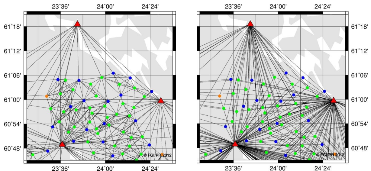
Figure 3. Alternative computation strategies of the test data. The data were processed as network (left) and individual (right) solutions. In the network solutions, adjacent points are mostly tied with a baseline in between. In individual solutions, all test points were tied only to the nearest three to four active GNSS stations, leaving the baselines between the test points unprocessed.
