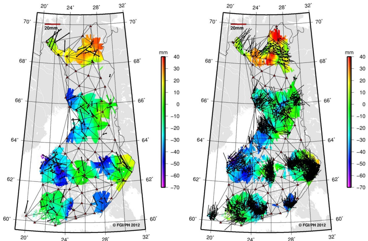
Figure 7. Residuals between coordinate classes. E1 residuals shown on the left and E2-E3 on the right. Horizontal residuals shown with black vectors and vertical with color map.
