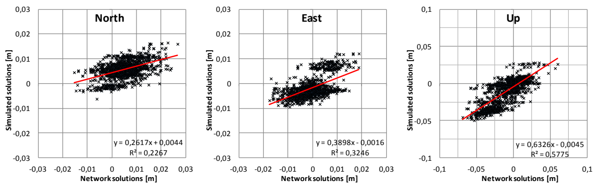
Figure 9. Correlation between network solutions and simulations for North (left), East (middle) and up (right) components. Results from three subnets including only one E1 point were eliminated from the correlation analysis. All E1 points have been removed as well because their residuals were used to propagate simulated residuals for other points in the networks and the correlation for E1 points therefore is equal to 1.
