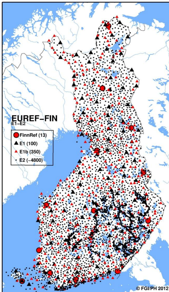
Figure 1. Finnish ETRS89 realization, EUREF-FIN, and its nationwide densifications (E1-E2).
