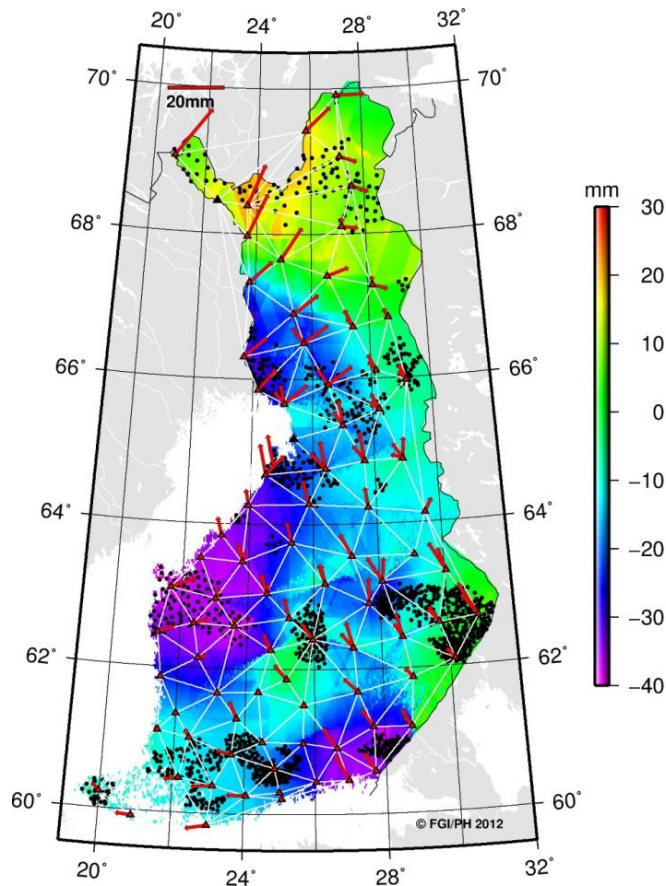
Figure 10. Simulated biases for the VRSnet.fi stations. The biases can only be considered as indicative. If the station has more than one bias, it has been a fiducial station in more than one subnet.
