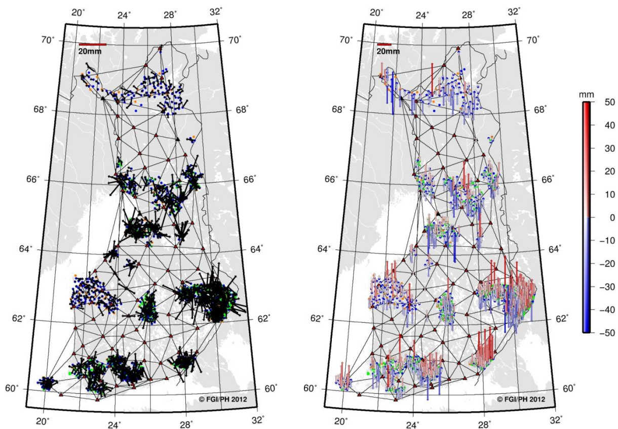
Figure 5. Difference between the solutions (individual minus network solution). Horizontal differences shown on the left and vertical on the right (note different scale in horizontal and vertical plots).
