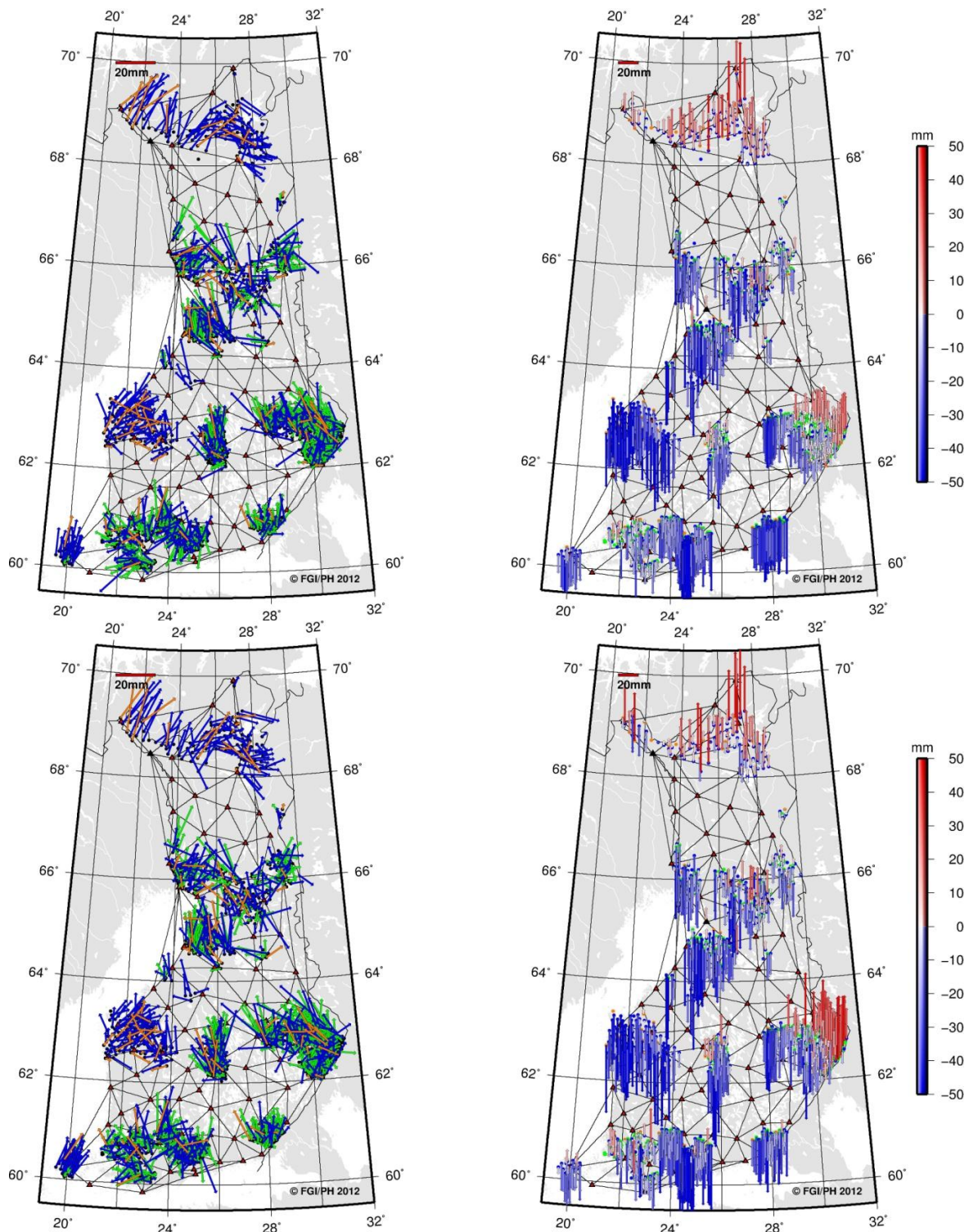
Figure 4. Accuracy of network solutions (top figures) and individual solutions (bottom figures). Horizontal residuals shown on the left and vertical on the right (note the different scale in horizontal and vertical plots). In horizontal plots, E1 residuals are shown with orange colour, E2 with blue and E3 with green.
