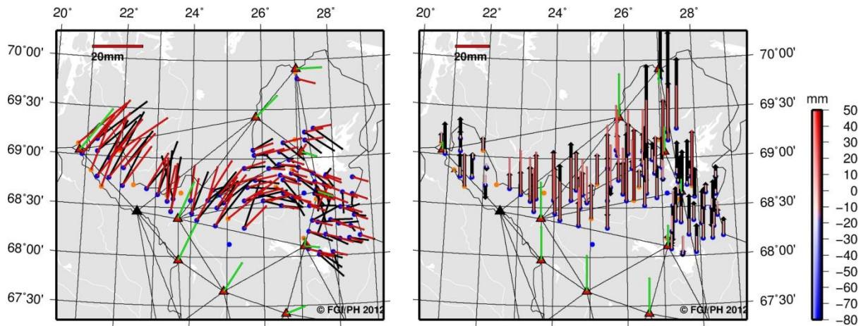
Figure 8. Snapshot of comparison of network and simulated solutions. On the left horizontal and on the right vertical residual (note different scale). Black vectors indicate residuals from the network solution and red or colored vectors are simulated residuals. Simulated residuals for VRSnet.fi stations are shown with green vectors. A black triangle indicates one VRSnet.fi station from where the data were unavailable for the study period.
